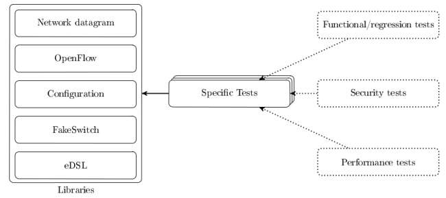
Figure 1: The hprobe architecture
